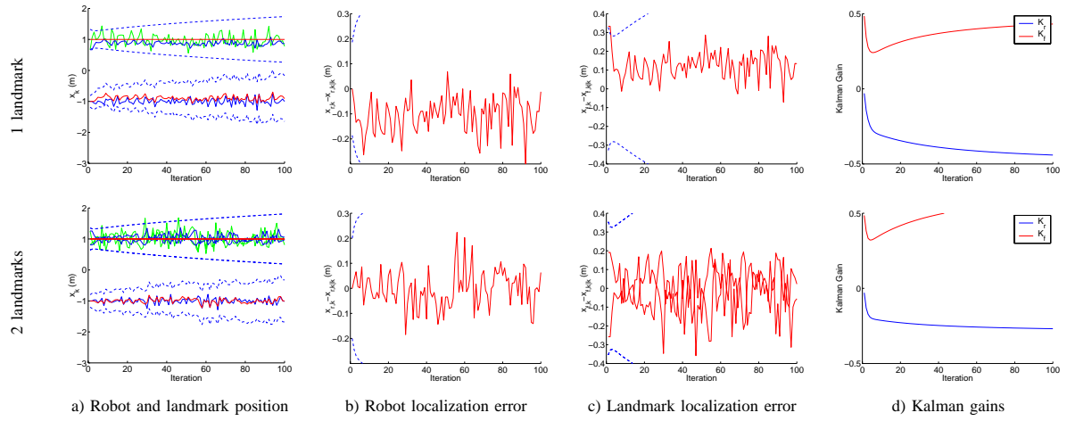
Fig. 2. Partially observable SLAM for a Brownian motion monobot with 100 iterations. The entire state error covariance is decorrelated with the minimal trace solution [5]. By decorrelating the entire state error covariance matrix, the covariance estimates become unbounded.
