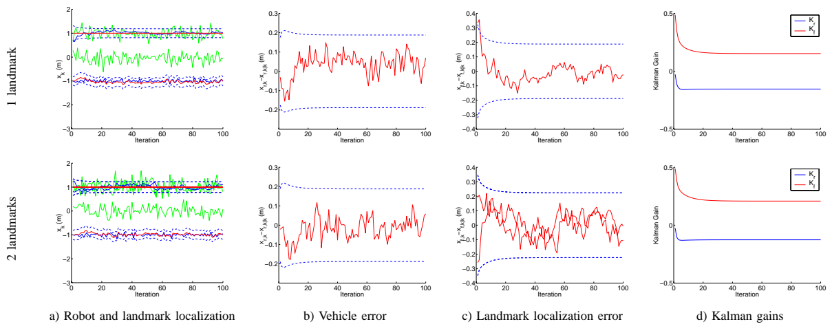
Fig. 4. Fully observable SLAM for a Brownian motion monobot with 100 iterations. The entire state error covariance is decorrelated with the minimal trace solution. In the linear case, it is possible to decorrelate the entire state error covariance matrix, and still preserve filter stability.
