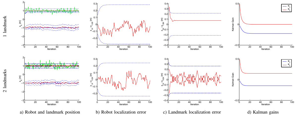
Fig. 3. Partially observable SLAM for a Brownian motion monobot with 100 iterations. The state error covariance is decorrelated only for the landmark part of the state vector, with the minimal trace solution. By decorrelating only the map part of the state error covariance matrix, we preserve filter stability.
