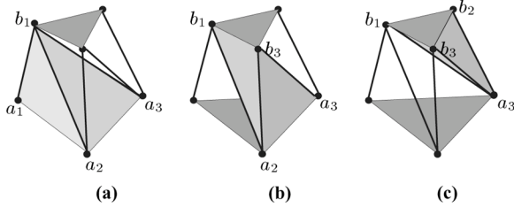
Fig. 5. Tetrahedra involved in the computation of the forward kinematics of the parallel manipulator in Fig. 4(b).
