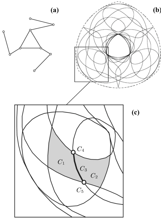
Fig. 1. (a) 3-RRR planar parallel manipulator. (b) Its singularity locus for a constant orientation is the root locus of a polynomial of degree 42 (adapted from [3]). (c) Then, the configuration space of the manipulator can be stratified into cells of strictly diminishing dimension.
