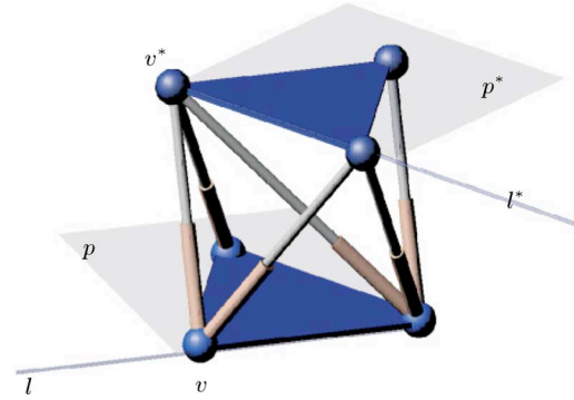
Fig. 6. Basic flagged manipulator and its attached flags.
