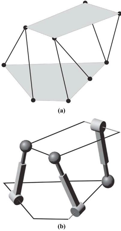
Fig. 12. (a) 2-1-1-2/1-1-2-1-1 manipulator and (b) a three-legged flagged manipulator derived from it by substituting the three two-leg groups by PRPS serial chains satisfying the required alignment on the base.
