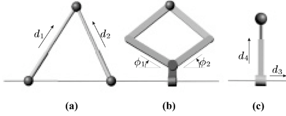
Fig. 11. (a) Two-leg group can be substituted, for example, by (b) a pantograph or (c) a PRPS serial chain.
