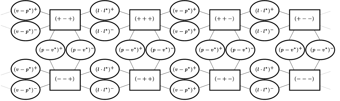
Fig. 16. Graph showing the topology of C-space for flagged manipulators. The rectangles represent the 6-D cells of C-space nonsingular configurations which correspond to the eight different assembly modes, while the ellipses are the 5-D cells of singular configurations.
