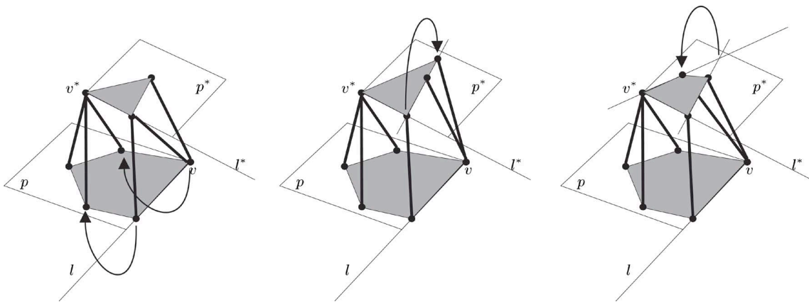
Fig. 10. 3/2 Hunt-Primrose manipulator is a flagged manipulator because it can be obtained by applying a sequence of four local transformations to the basic flagged manipulator. Notice how the attached flags remain invariant under these transformations.
