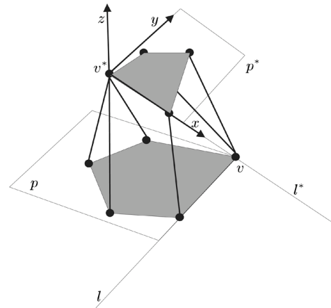
Fig. 3. Singular configuration of a 3/2 Hunt–Primrose manipulator, in which two of the tetrahedra defining its forward kinematics are degenerate.
