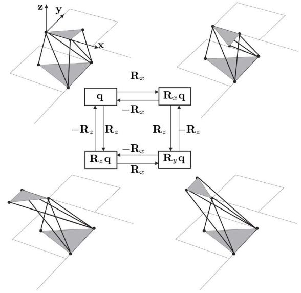
Fig. 15. Four platform configurations sharing the same flag, obtained by rotating \pi radians about its reference axes.
