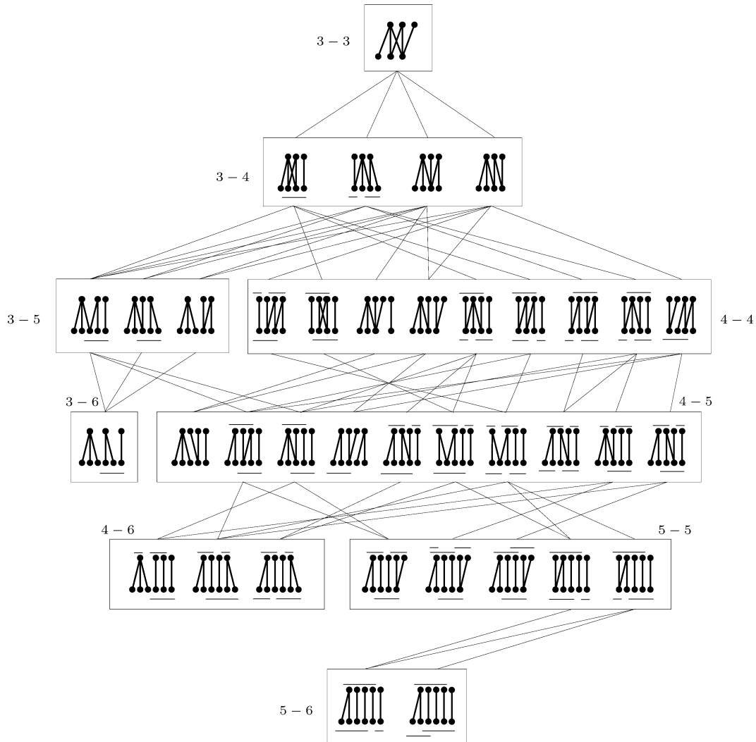
Fig. 9. Whole family of six-legged flagged manipulators expanded from the basic one by applying the transformation in Fig. 8(a). Segments, next to either the base or the platform, indicate the endpoints that should be kept aligned.
