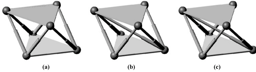
Fig. 4. Three possible architectures for the 3-3 parallel manipulators.
